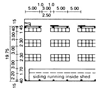
⑦ Plan view, cross-section → ④ type D
